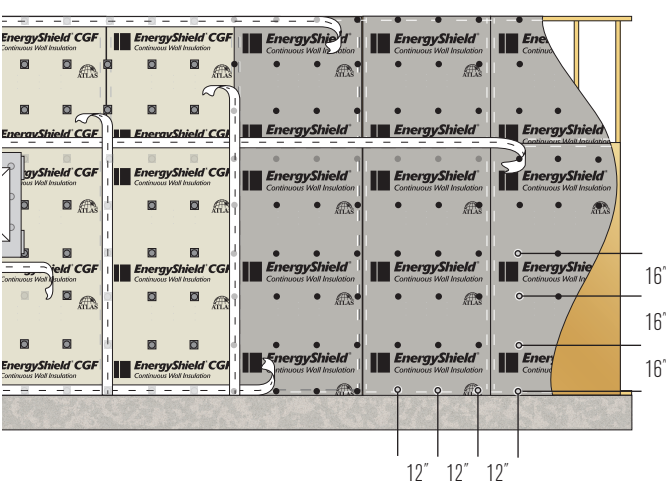
FIGURE B: FOAM BOARD AS CONTINUOUS INSULATION AND WRB OVER EXTERIOR WOOD SHEATHING FASTENED TO WOOD STUD FRAMING
