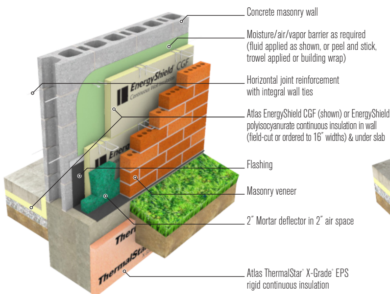
IMAGE 3: MASONRY CAVITY WALL WITH EXTERIOR CONTINUOUS INSULATION
