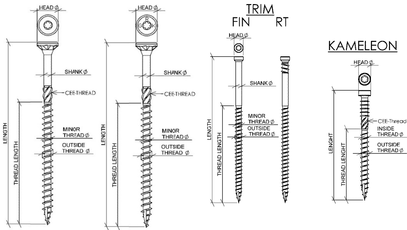
FIGURE 1—GRK SCREWS
