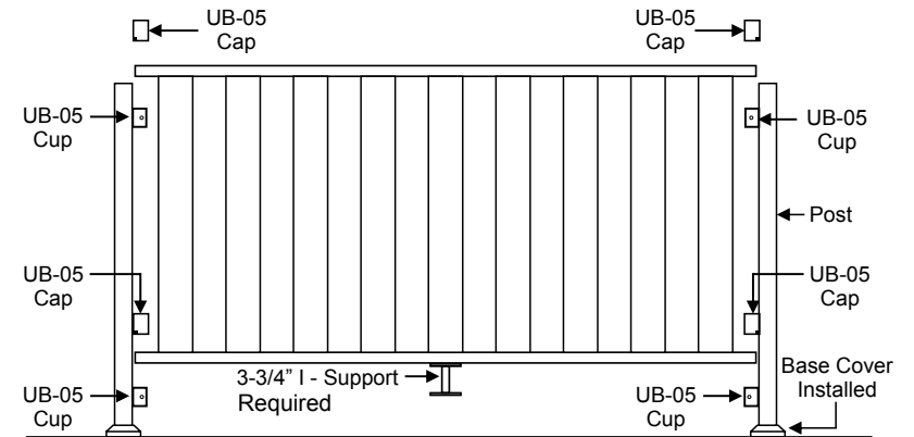
Universal Brackets
