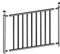
Maximum Overall width 48" (1219mm)
