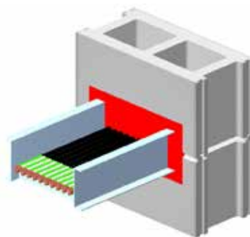
Typical Cable Tray Penetration
