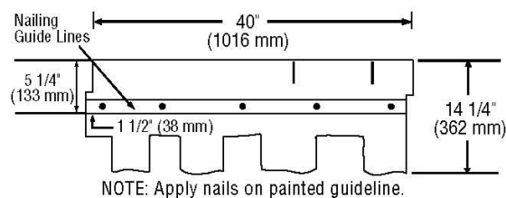
NOTE: Apply nails on painted guideline. Figure 16-6: Fastening Presidential and Presidential TL Shake shingles on low and standard slopes.
