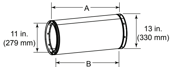
Chimney Sections
