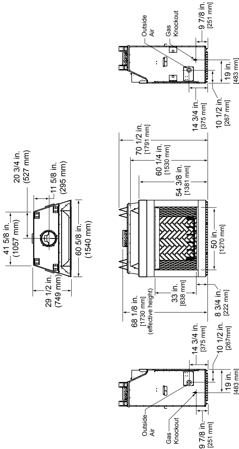
Figure 3.1 Fireplace Dimensions
