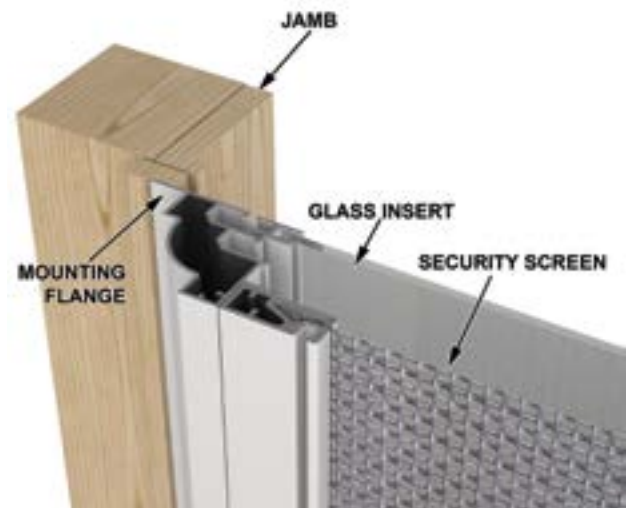
Storm Window – Overlap Application
