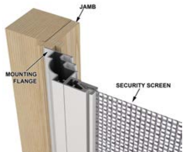
Screen Window – Overlap Application
