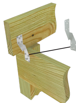
Typical RT7A installation
