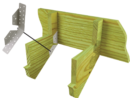
Typical CSH-TZ installation
