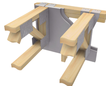
Typical FWH solid sawn header installation
