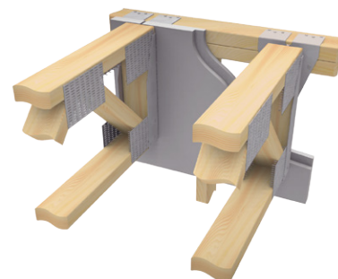
Typical FWH stud wall with (2) layers of 5/8" gypsum wall installation
