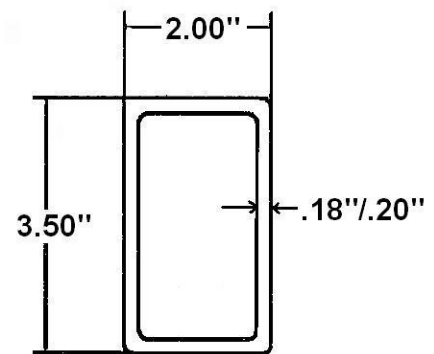
Bottom Rail (1)
