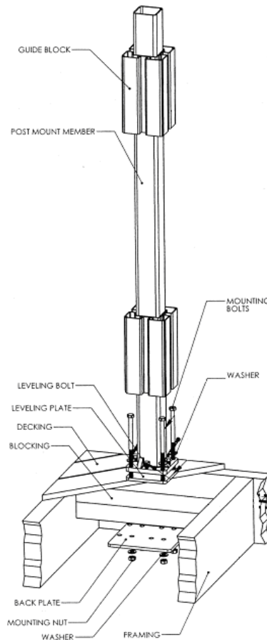
FIGURE 9 – TAM-RAIL® OR MARQUEE™ POST MOUNT SYSTEM WITH PVC GUIDES
