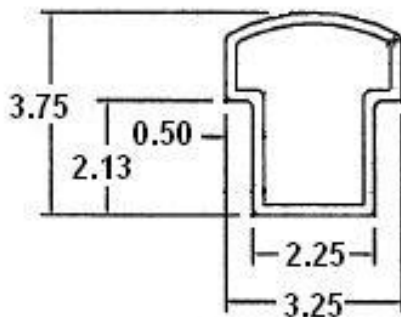
Upper T-Rail (1)
