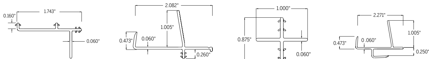
BRICKMOULD CONNECTOR
